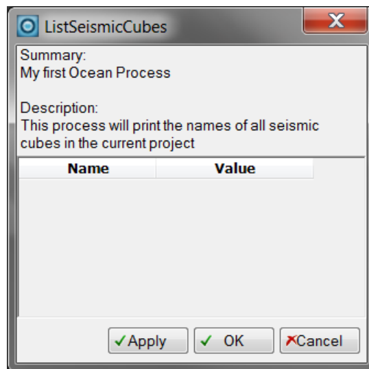
Figure 13: ListSeismicCubes Dialog
